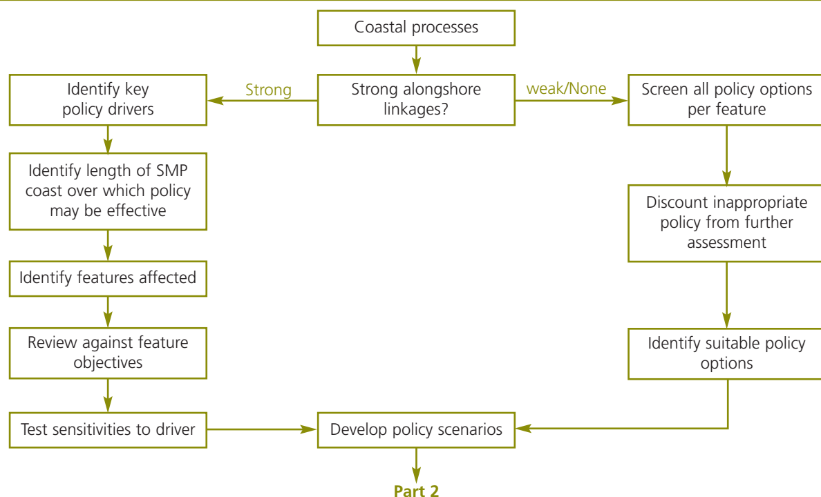
Figure 3.0 Stage 3 Flow diagram; Part 1: Task 3.1
