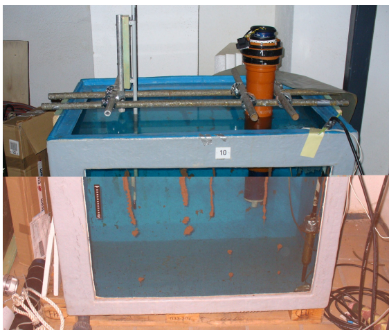
Fig. 2-17: Testtank setup
