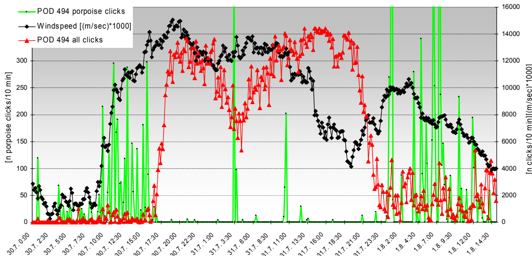
Fig. 2-10: Wind speed, all recorded clicks and harbour porpoise click trains identified by the algorithm of T-POD 494 in the time period July, 30th to August, 1st (extraction of fig. 33)
