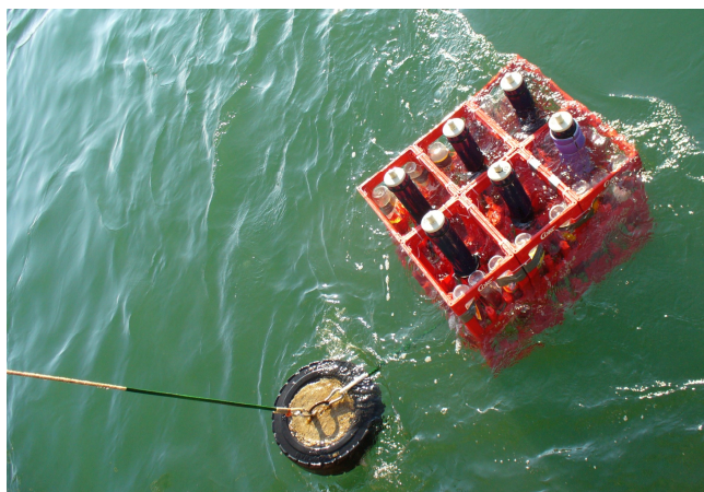
Fig. 2-18: Plastic frame for inter calibration experiments with 6 T-PODs during recovery.
