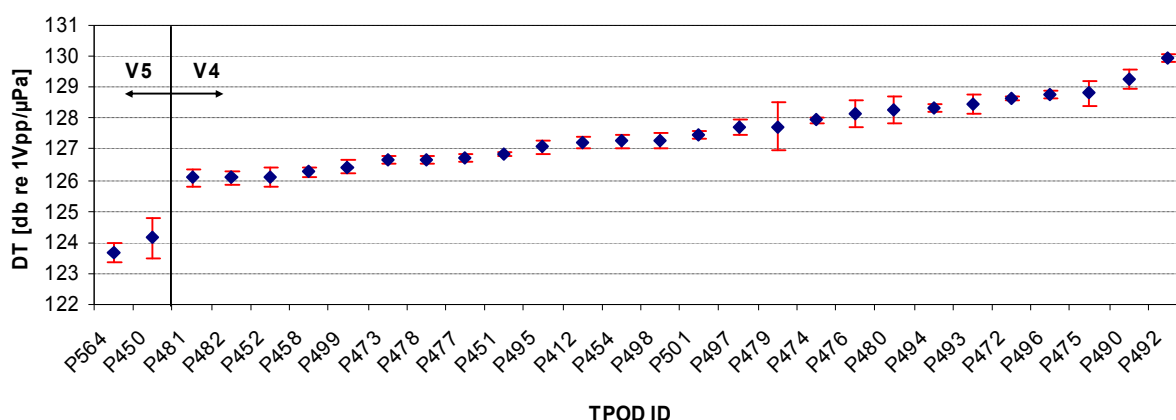
Fig. 2-19: Absolute detection thresholds (dB re 1Vpp/μPa) of all T-PODs used in this study with standard settings. The accuracy of measurement is about 2 db.
