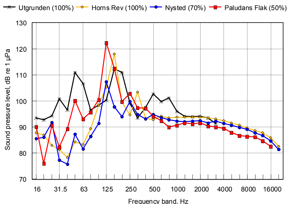
Fig. 2-5: Spectra from Fig. 2-4 in third-octave representation.
