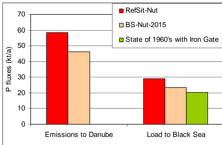
Figure 34: Phosphorus emissions for the Reference Situation-Nutrients (RefSit-Nut), Baseline Scenario-Nutrients 2015 (BS-Nut 2015) and the situation in the 1960s. 83
