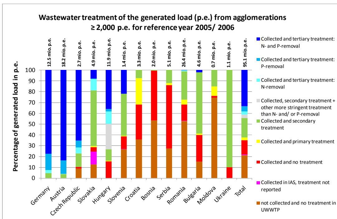
Figure 3: Existing wastewater treatment plants; existing treatment levels and degree of connection to wastewater treatment for the entire DRB by country. 26
