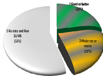
Figure 24: Ecological potential for AWB (incl. share of Non EU MS providing provisional designation) in relation to total number of water bodies.
