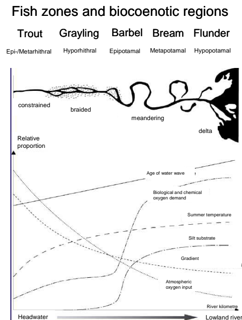
Figure 36: Definition of fish zones and rhithral (headwater) and potamal (lowland river) sections.
