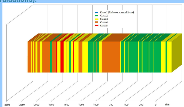
Figure 11: Overall hydromorphological assessment of the Danube River in five classes as longitudinal colour-ribbon visualisation. 44
