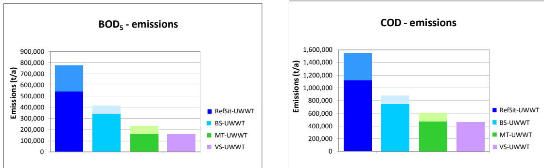
Figure 29: Emissions of BOD 5 and COD for the Reference Situation UWWT (RefSit-UWWT) and the three different scenarios (Baseline Scenario-UWWT 2015; Midterm Scenario-UWWT; Vision Scenario-UWWT). [The lighter coloured parts of the columns represent wastewater emissions that are not collected in sewerage systems and not treated in a wastewater treatment plant.]
