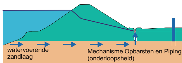
Figure 2-8 Mechanism of uplifting and piping in dikes
