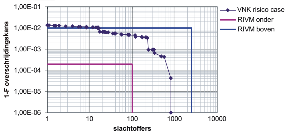
Figure 3-11 Group risk curve for dike ring 36 and comparison with RIVM estimates
