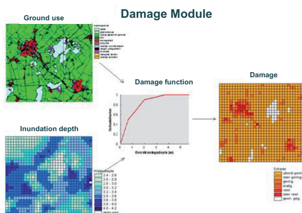
Figure 2-3 Flow diagram for damage calculation
