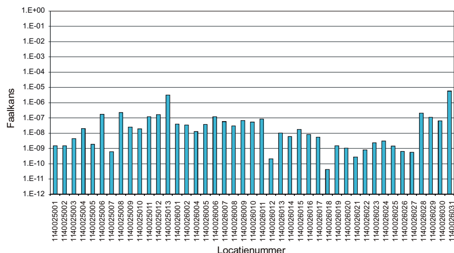
Figure 3-3 Probability of failure of the dike sections in dike ring 14: Zuid-Holland for the mechanism overflow or wave overtopping.
